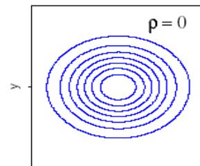
No covariance
