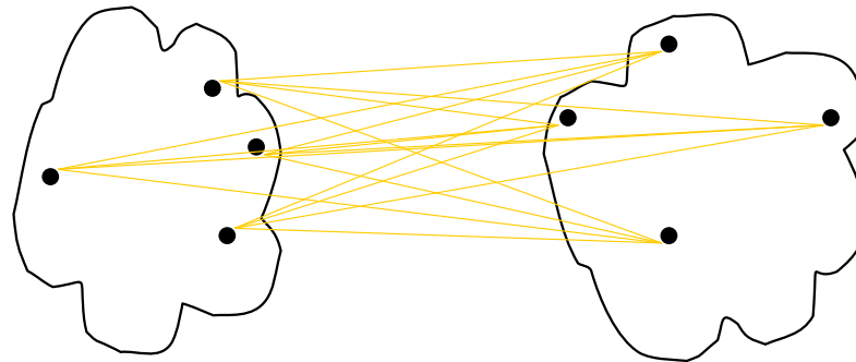
separation
