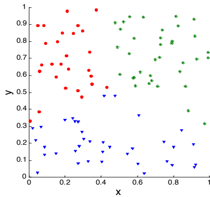
K-means
