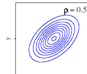
Positive covariance
