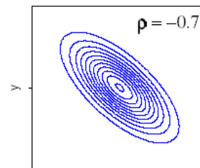
Negative covariance
