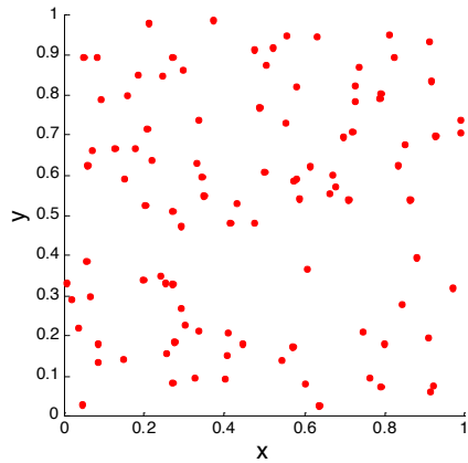
Random Points
