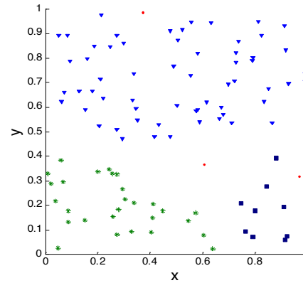
DBSCAN
